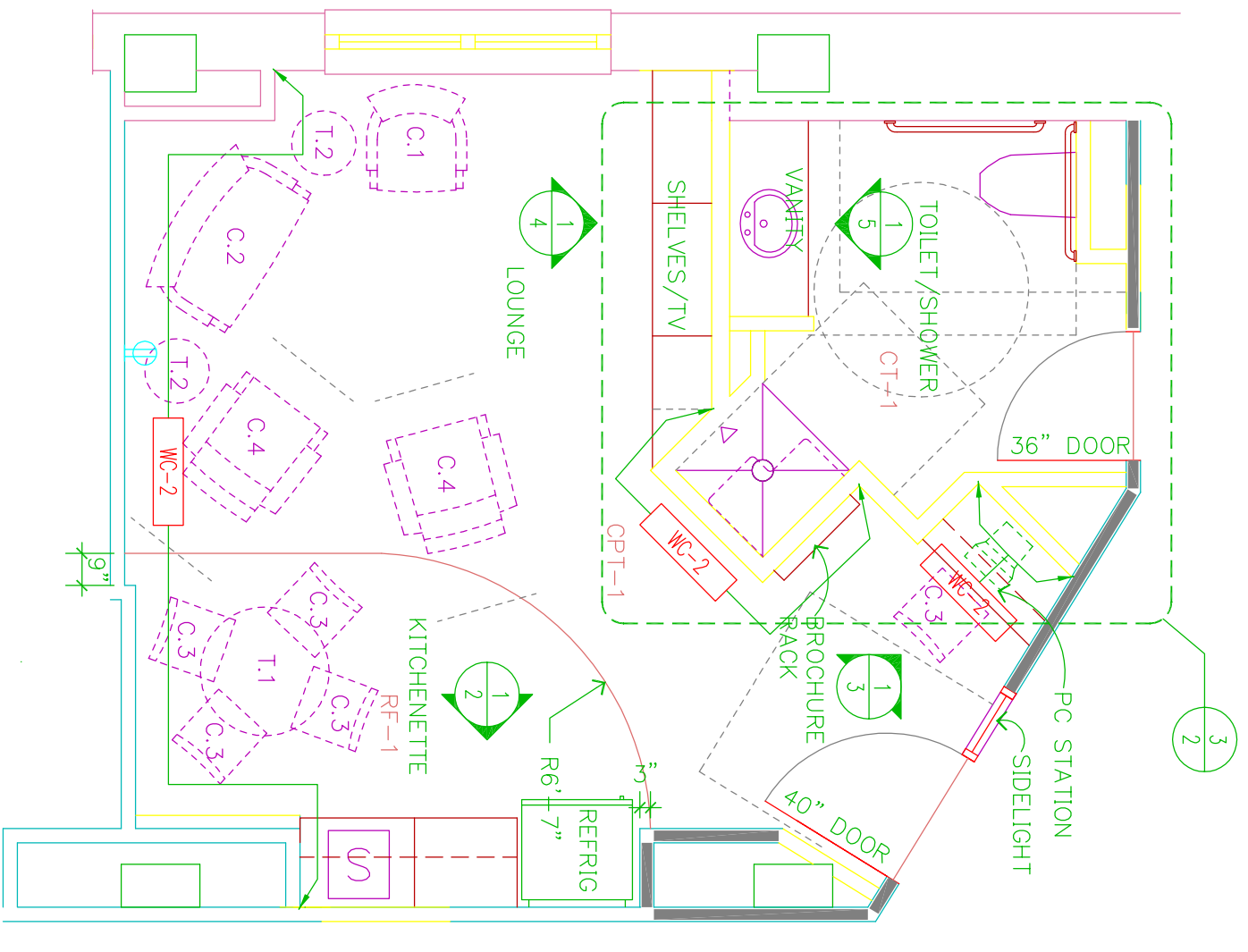
1 PLAN
